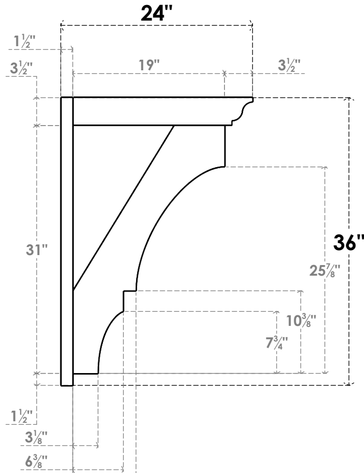
SIDE PROFILE
